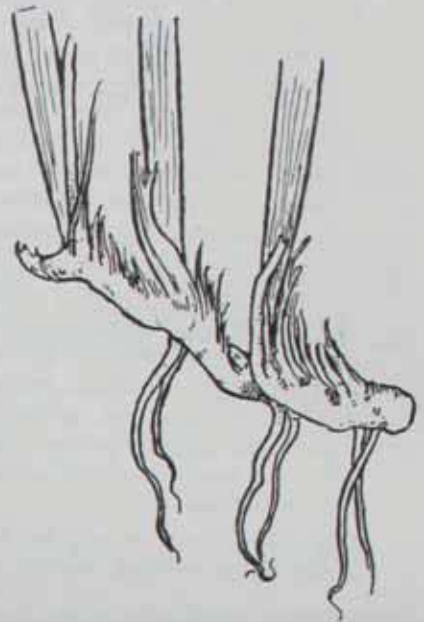
FIG. 4. The rhizome of I. bracteata .
