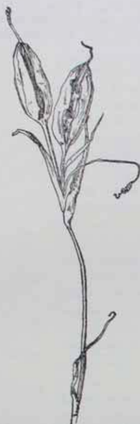
FIG. 15. Inflorescence of I. flavissima , showing two capsules and one withered flower that failed to set seed.
