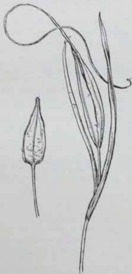
FIG. 30. Spathes, capsule, and withered perianth tube of I. reticulata , and capsule of I. Danfordiae .
