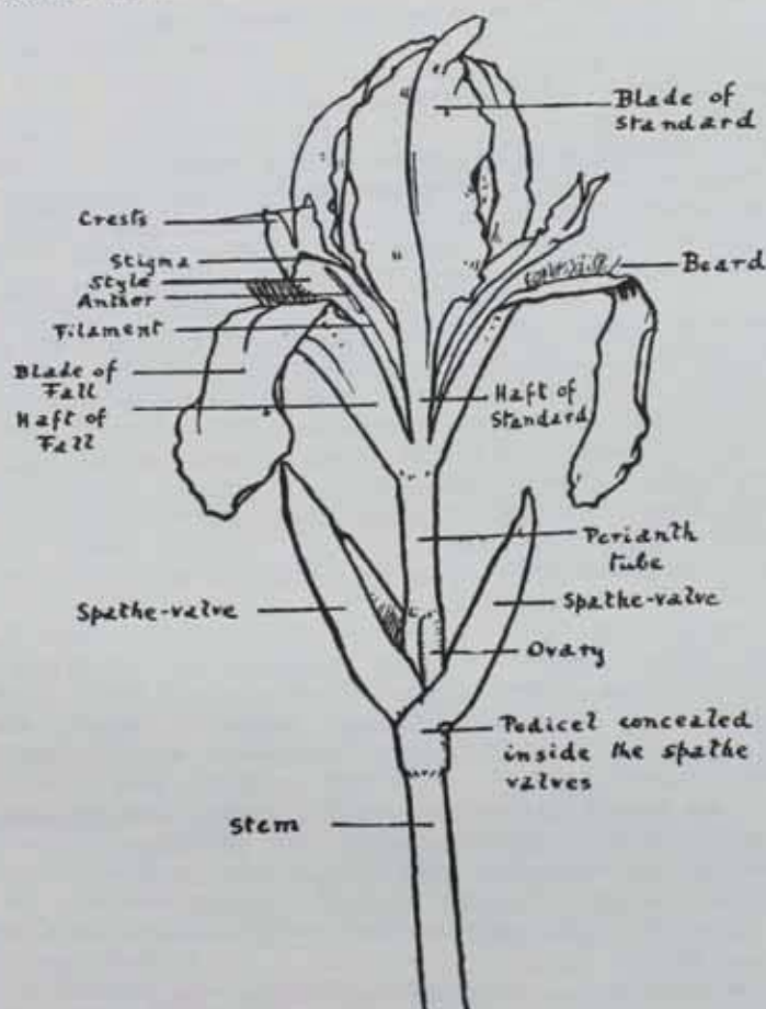
FIG. 1. Structure of the Iris flower.
