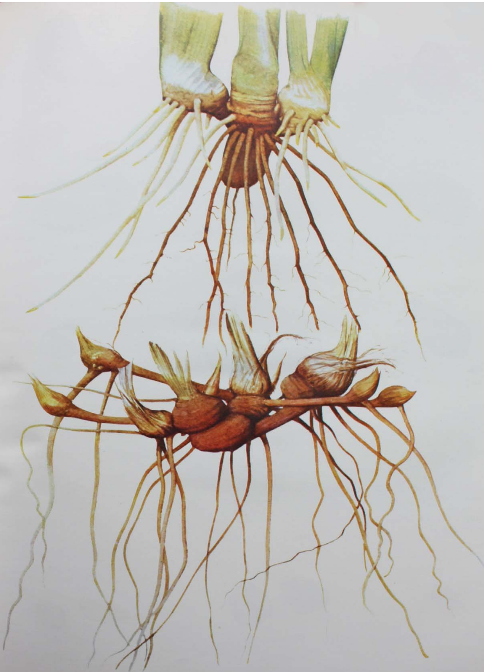
PLATE XLVII Rhizomes of a Pogoniris and of a Regelia Iris
