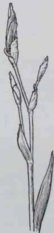
FIG. 21. Typical inflorescence of I. germanica ; much reduced.
