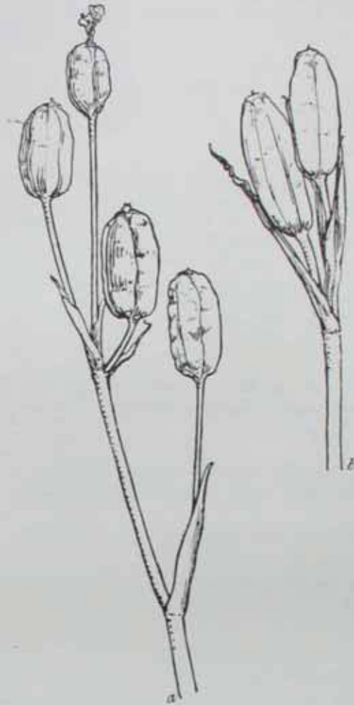
FIG. 2. Ripe capsules of (a) I. sibirica , (b) I. orientalis .
