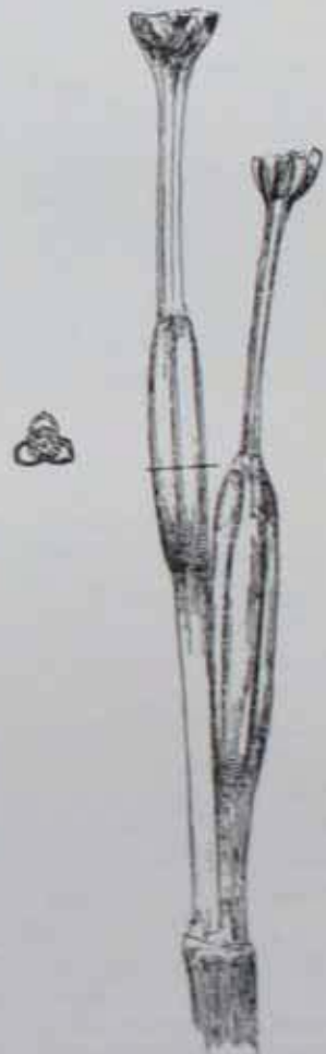
FIG. 29. The inflorescence of I. tingitana , showing the long perianth tube.
