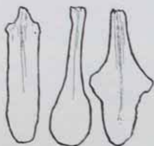
FIG. 26. The three types of outer segment in the Juno section.
