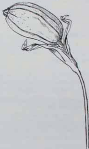
FIG. 10. Capsule of I. fulva (slightly reduced).
