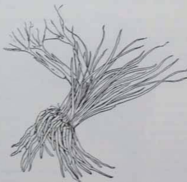
FIG. 18. I. tigridia from a herbarium specimen; half the natural size.
