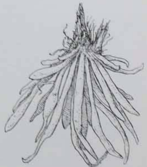
FIG. 25. Rootstock of I. nepalensis . Slightly reduced.
