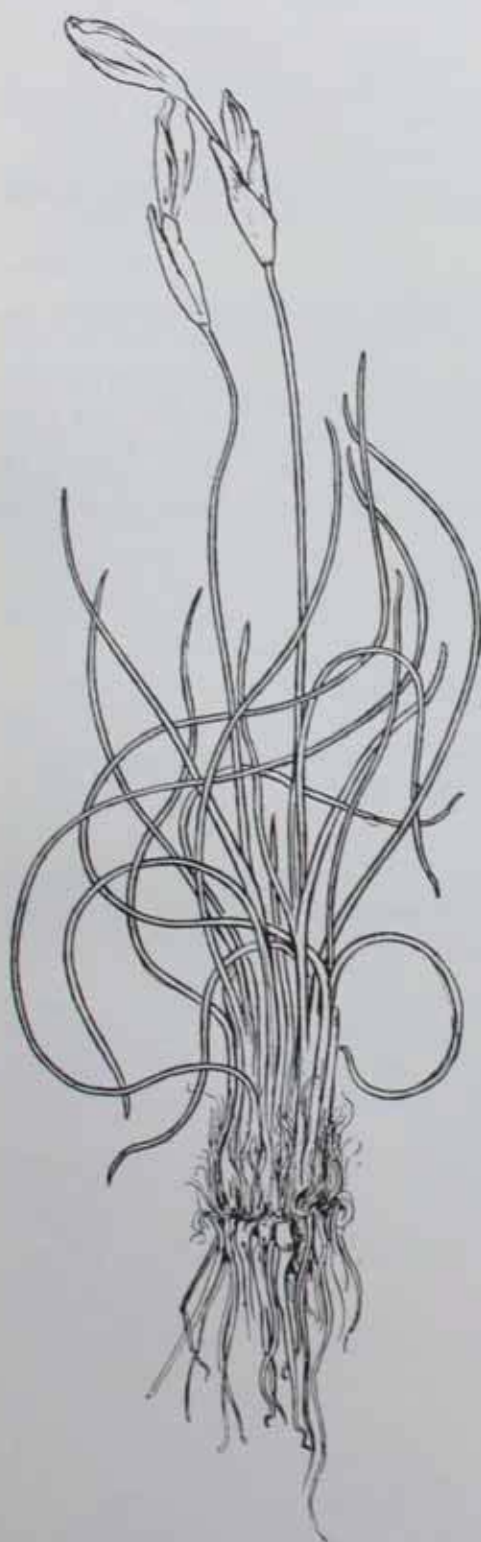
FIG. 14. I. falcifolia drawn from a herbarium specimen; about two-thirds of the natural size.
